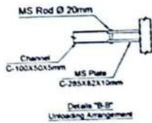
Details "B-B" Unloading Arrangement
