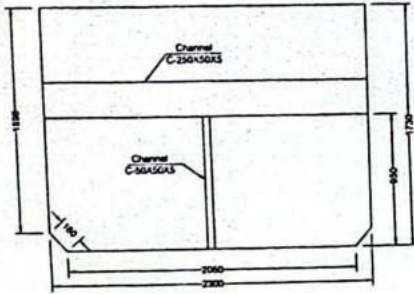
SECTIONAL VIEW 'AA'
