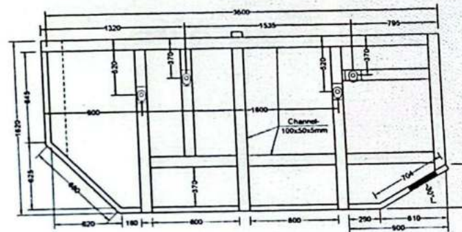
SIDE ELEVATION
